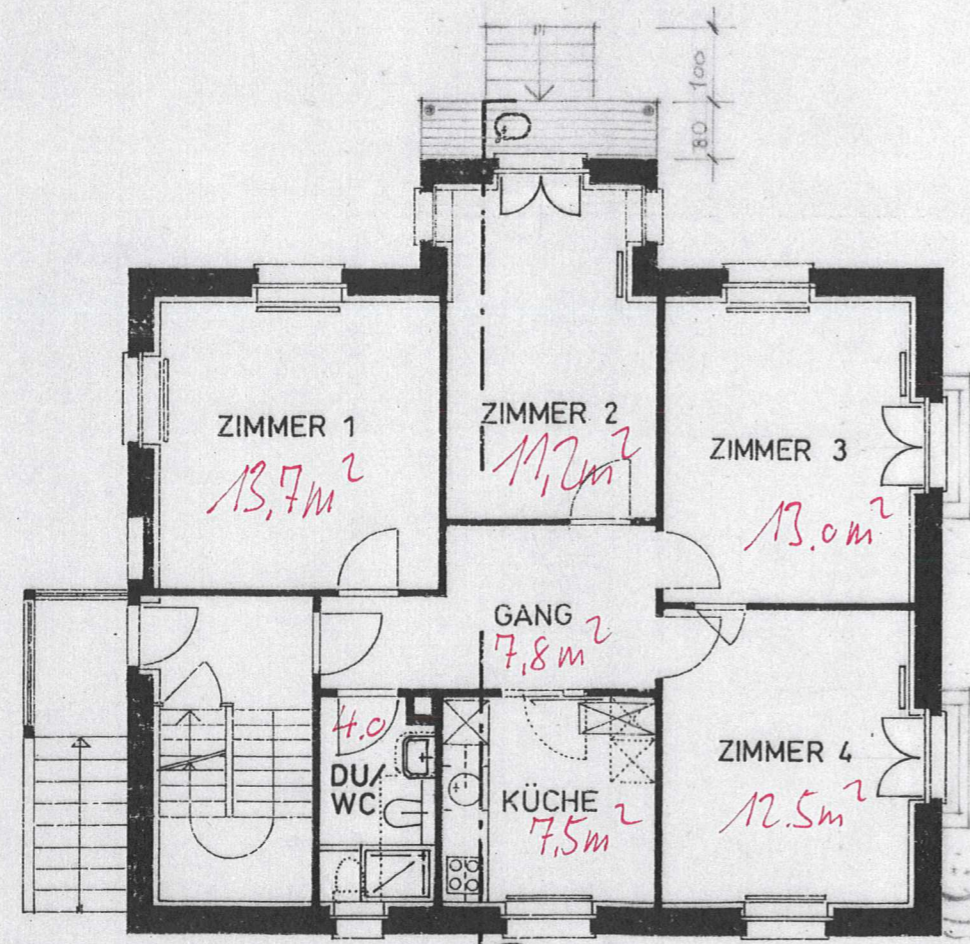
ERDGESCHOSS Total 69,7m 2
