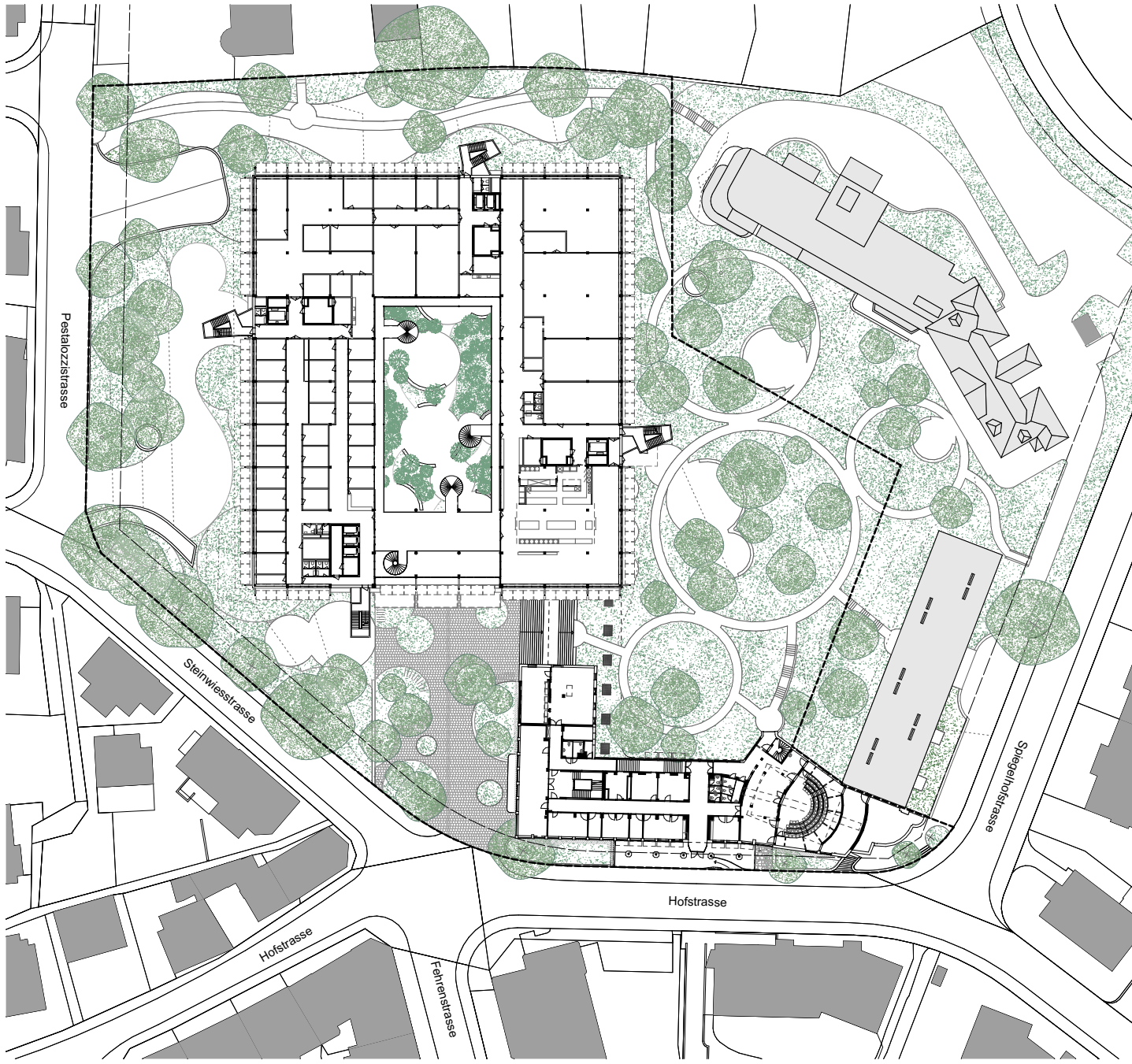
Situation M 1:1000
